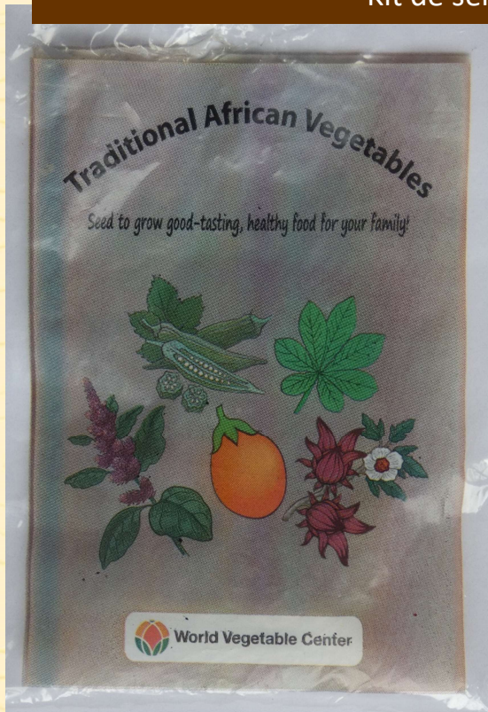
Photo face
