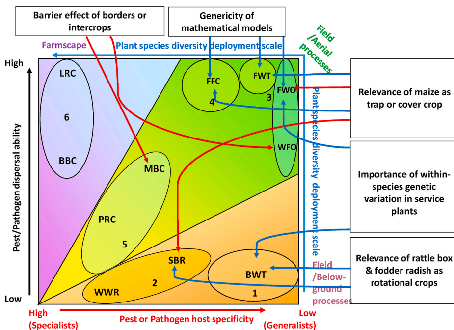
Fig. 1. Positioning of the reported case studies (cf. Table 1 for numbering and abbreviations), as a function of scale levels at which plant species diversity modalities and effects are deployed (field level via below-ground processes: bottom right triangle; field level via aerial processes: central kite; farmscape level: top left triangle), and a life history trait-based typology of pests and disease-causative pathogens (host specificity and dispersal ability), with some transversal synergies or tradeoffs highlighted. Blue arrow: positive regulatory effect on target pest/pathogen-crop system (synergy/genericity highlighted); Red arrow: negative (or absence of) effect (tradeoff requirement highlighted). (For interpretation of the references to color in this figure legend, the reader is referred to the Web version of this article.)
